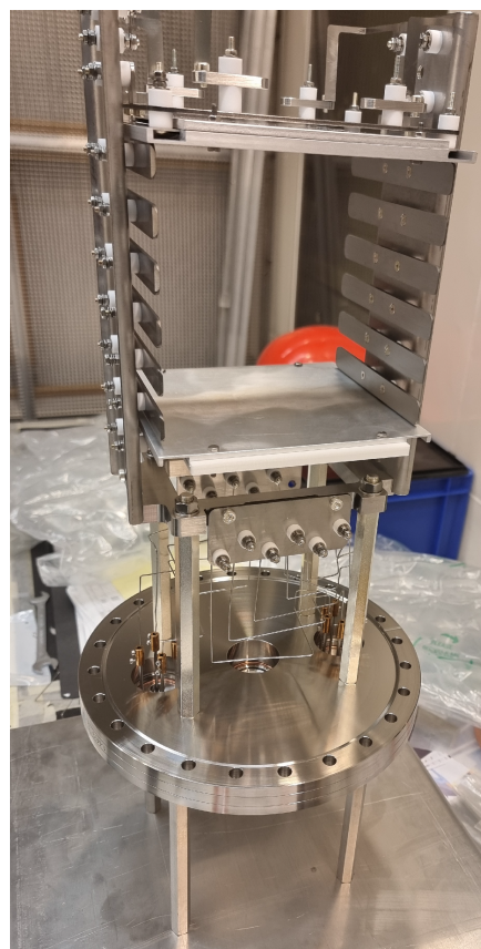
Figure 3: The ready mounted vacuum part of the IPM. On top a module with a MCP stack and a phosphor screen will be mounted. The E-field-box with its 6 field flattening electrodes is visible. On the bottom, covered with a protective shield during mounting, a fine mesh will be installed, which flattens the electric field but lets through UV light for calibration purposes. The UV light will be generated by a lamp mounted outside the vacuum, right behind the vacuum window in the lower CF flange.
